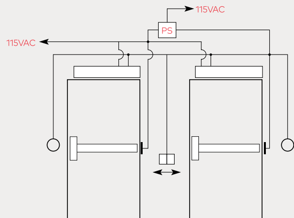
Latch Retraction
