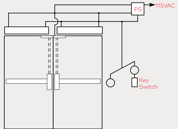
Electric Strikes
